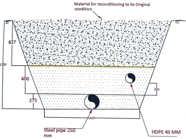
TRENCH IN NORMAL SOIL TYPICAL SECTION
