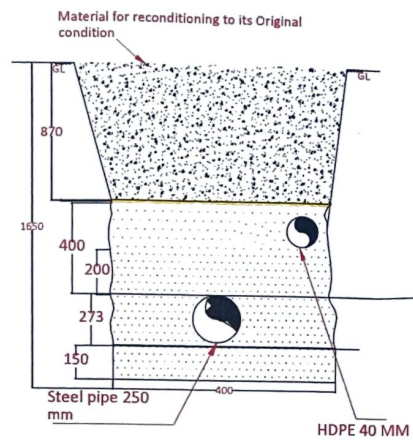
TRENCH IN CONSOLIDATED ROCK TYPICAL SECTION
